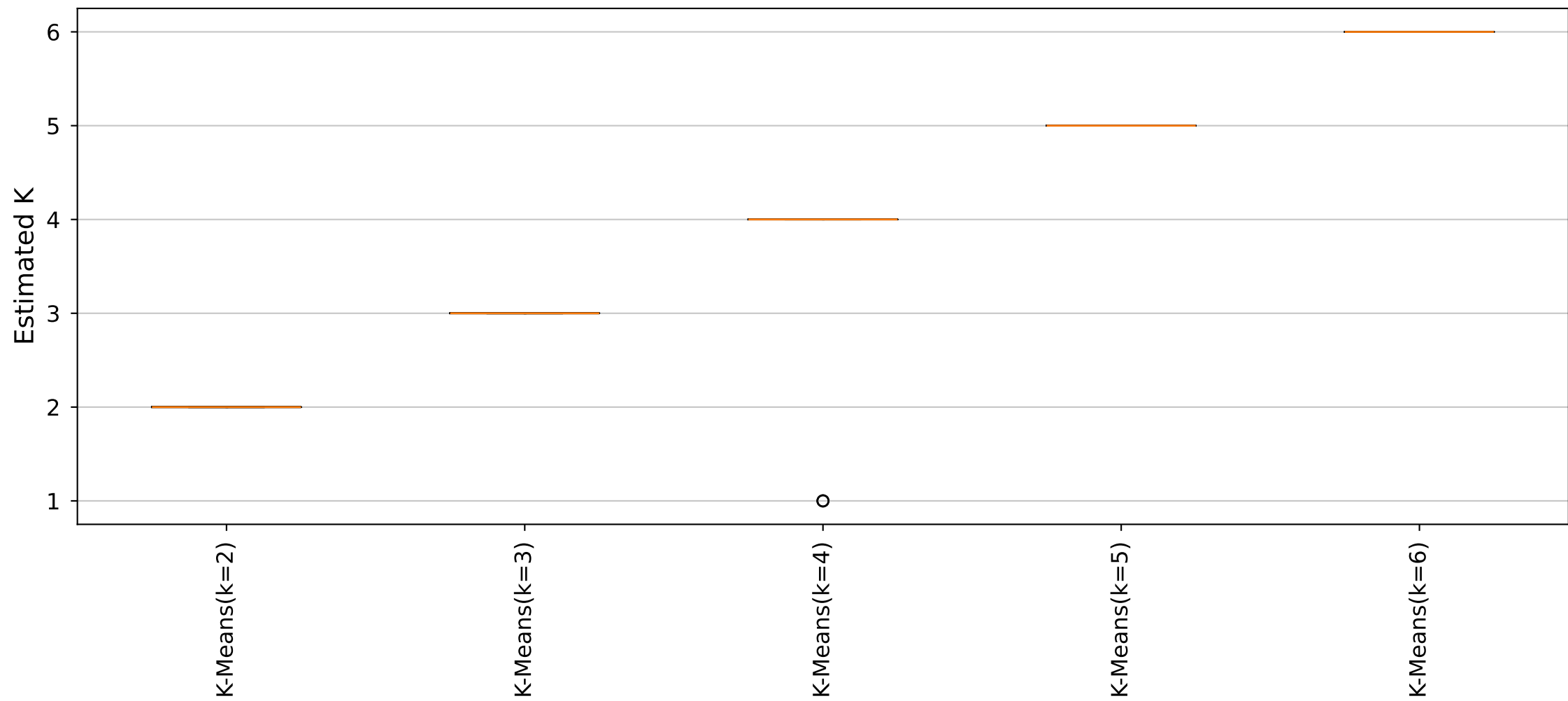
YARA Rules Estimated K Distribution (Cluster18_Size6 dataset)
